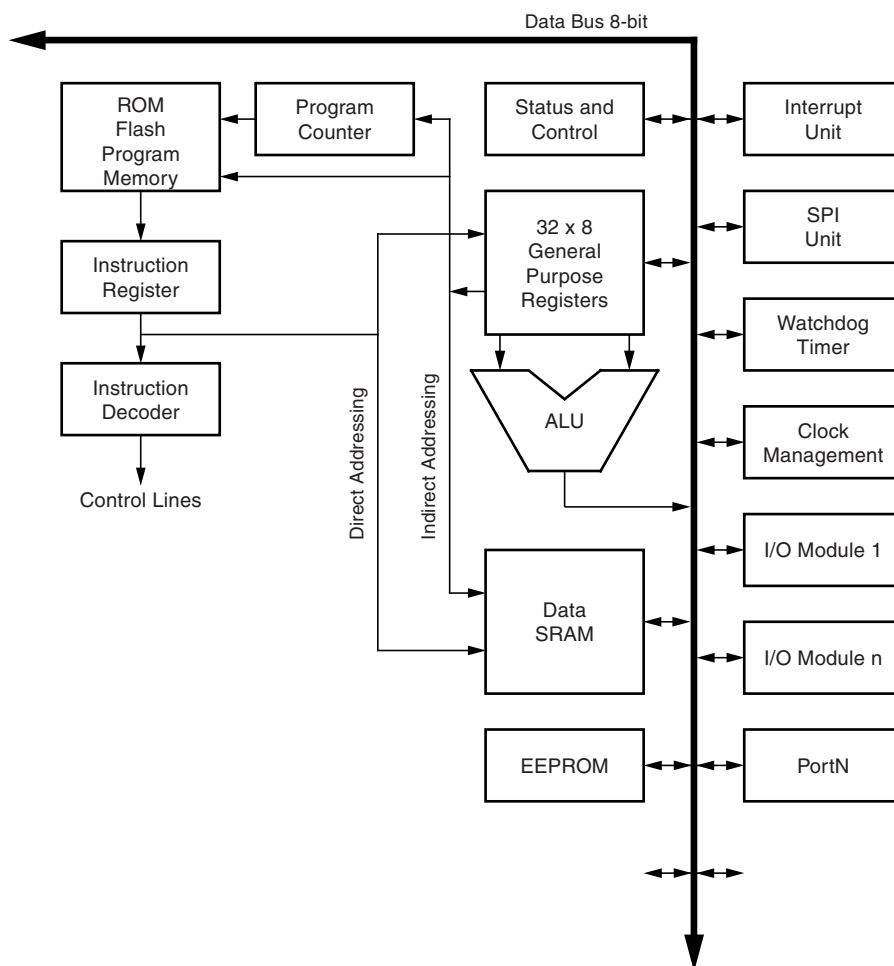
Figure 3-5. Architectural Overview
