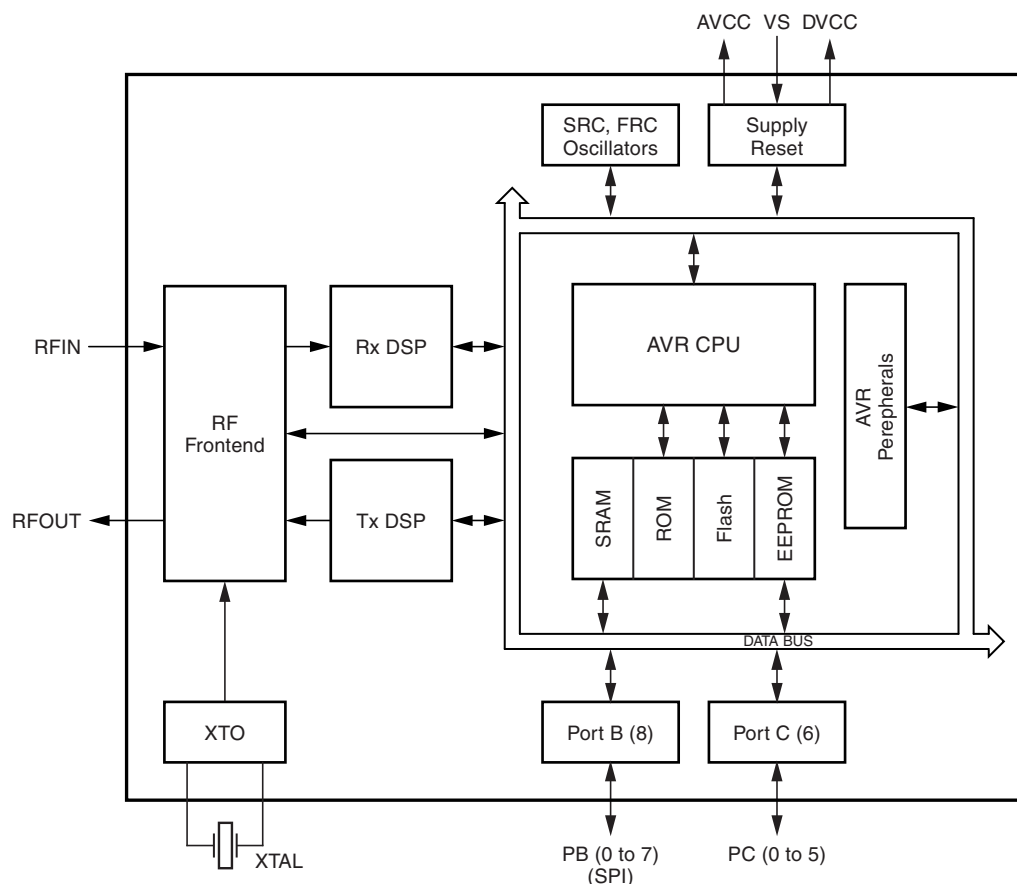
Figure 1-3. Circuit Overview
